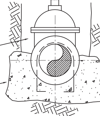
BURIED GATE VALVE APPLICATIONS
